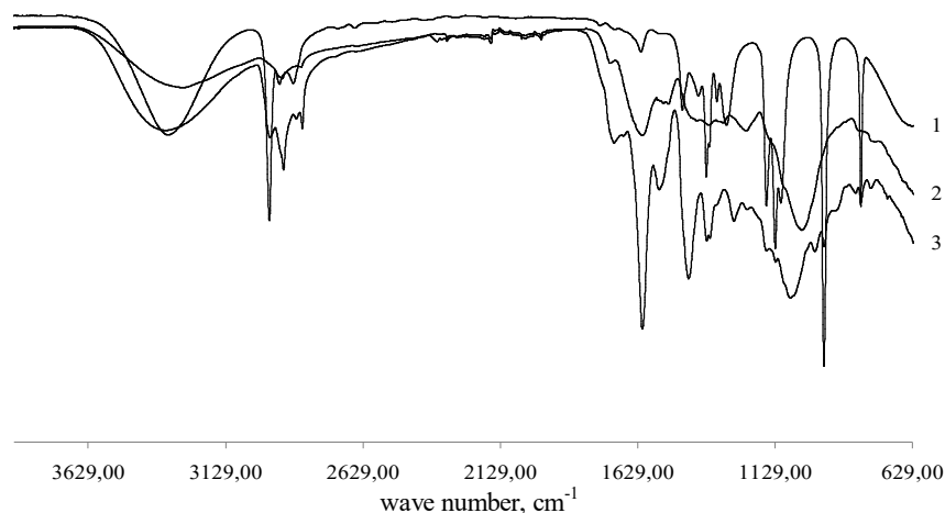
Fig. 4. Infrared attenuation spectra of corrosion products, obtained in 0.1M HCl solution without the inhibitors (1) and corrosion products, obtained after S3ps steel samples exposure to 0.1M HCl with In1 (2) and In2 (3)
