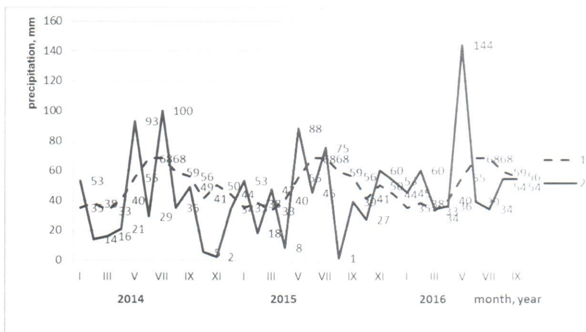
Figure 3. Dynamics of rainfalls in the city of Chernihiv for the period from January 2014 to September 2016. Legend: 1 - rate amount of precipitation for the month (mm), 2 - the actual rainfall for the month (mm) (the data of meteorological station "Chernihiv")
