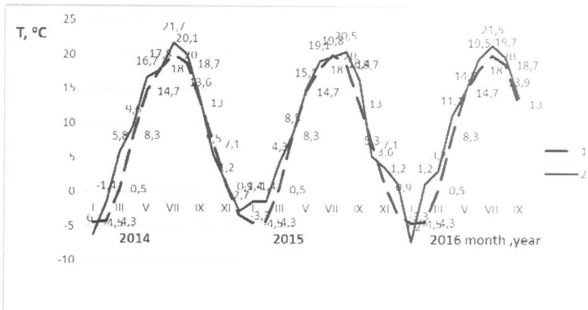
Figure 2. Dynamics of air temperature in the city of Chernihiv for the period from January 2014 to September 2016. Legend: 1 - average rate of temperature (°C), 2 - the actual average temperature (°C) (the data of meteorological station "Chernihiv")
